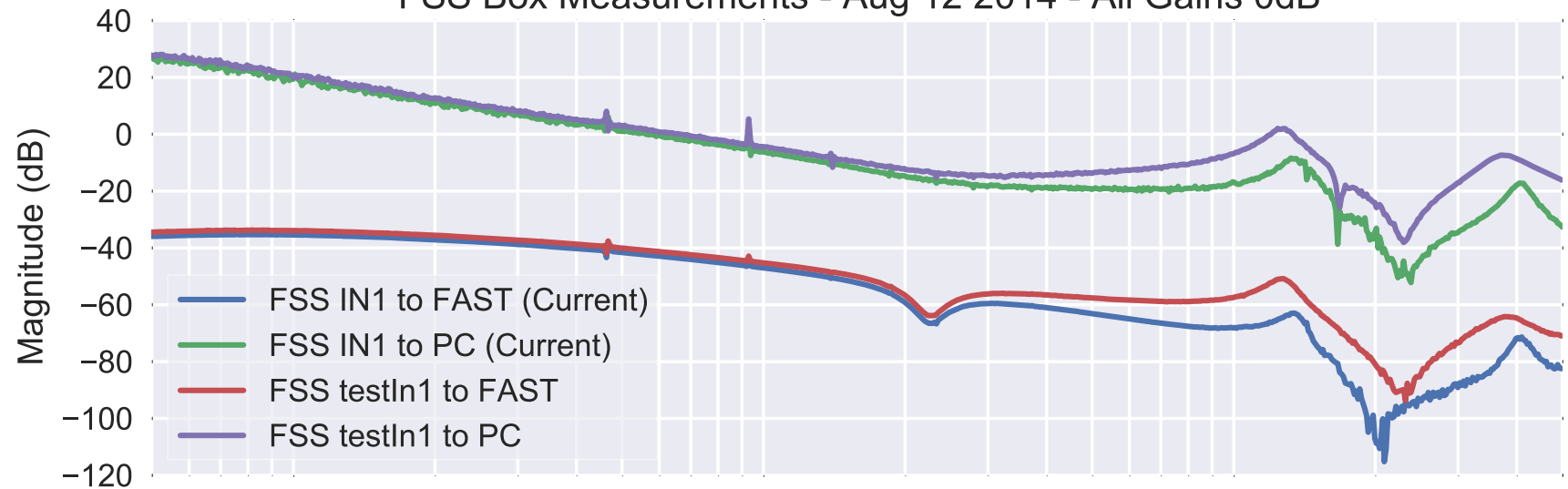
FSS Box Measurements - Aug 12 2014 - All Gains 0dB
