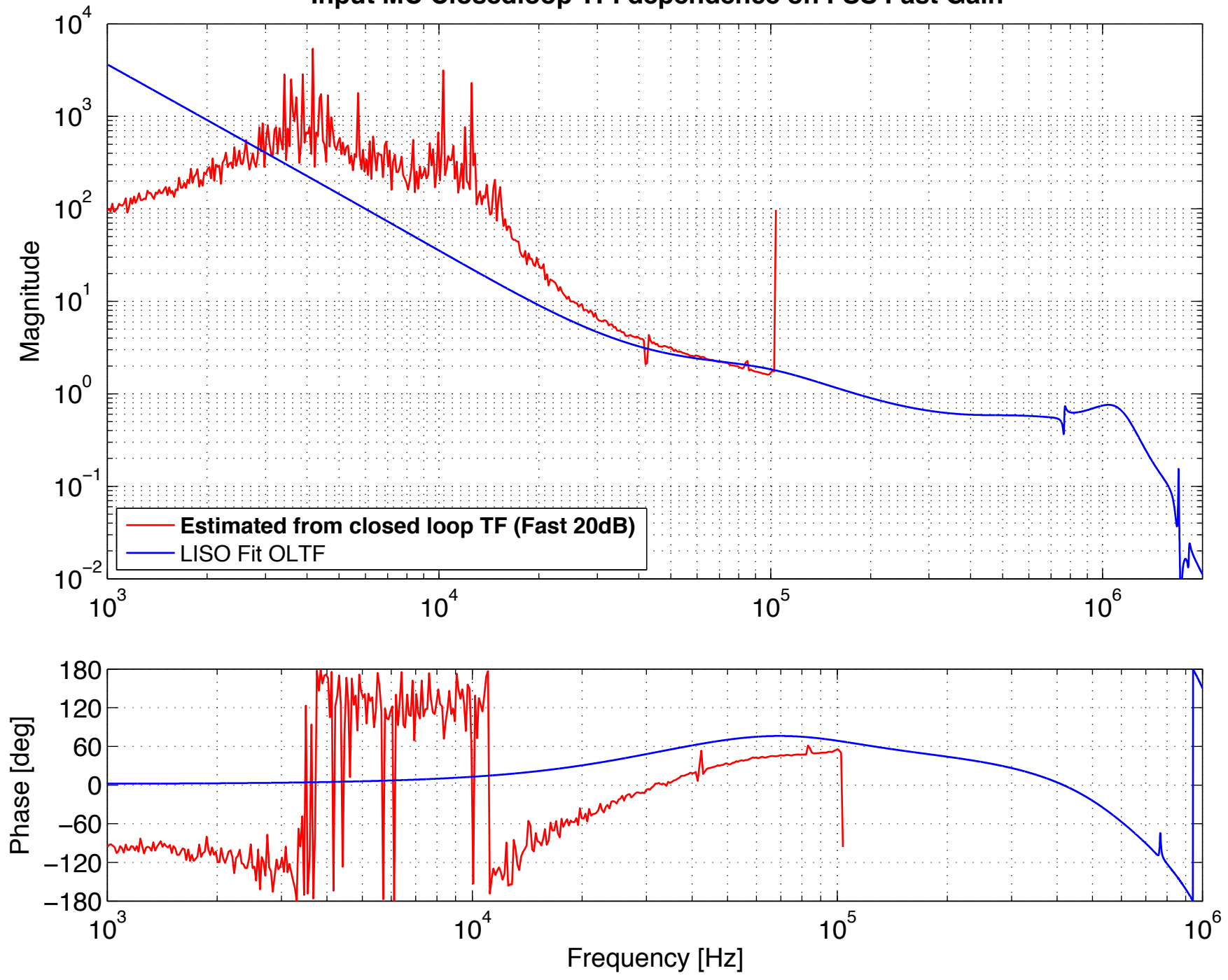
Input MC Closedloop TF: dependence on FSS Fast Gain
