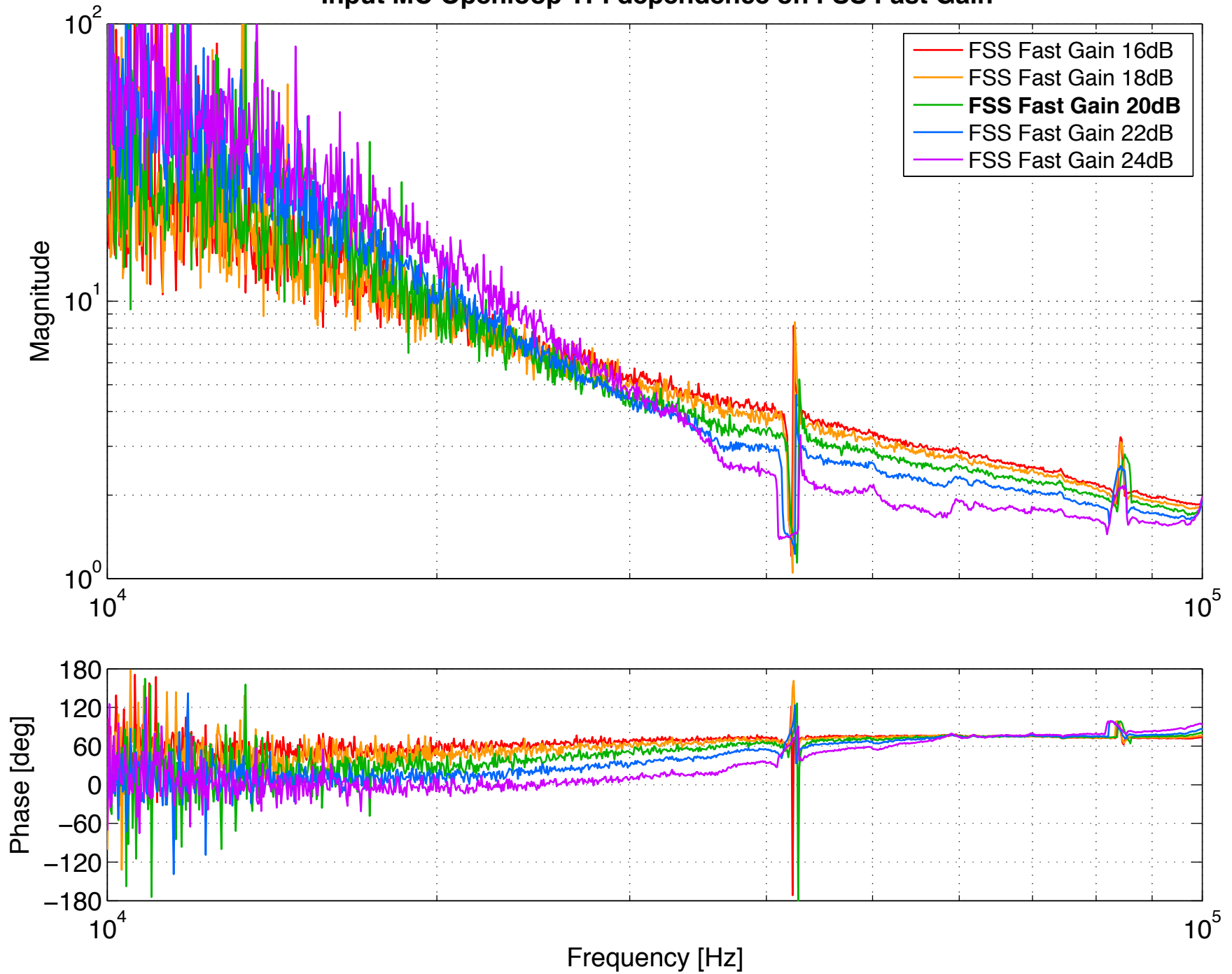
Input MC Openloop TF: dependence on FSS Fast Gain
