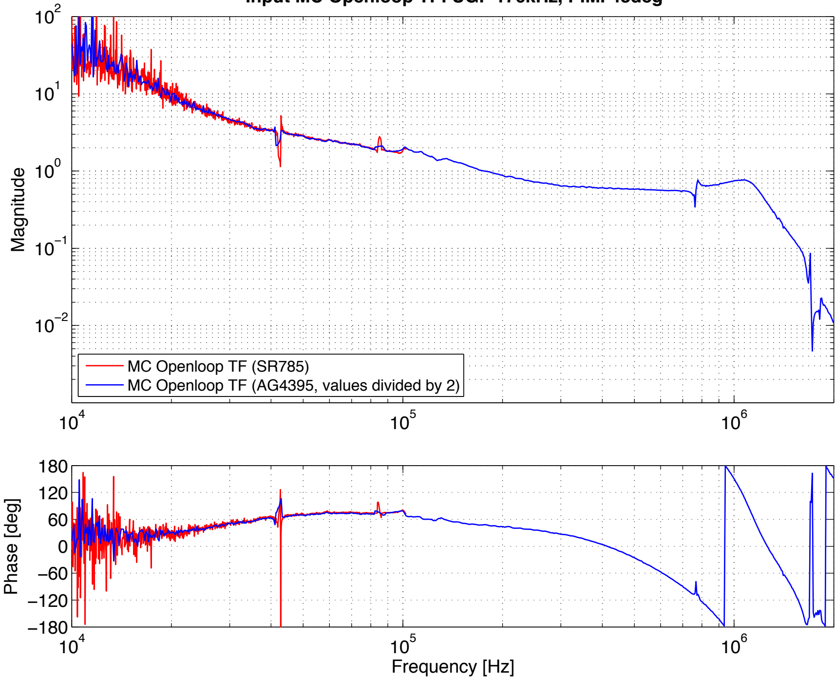
Input MC Openloop TF: UGF 176kHz, P.M. 48deg
