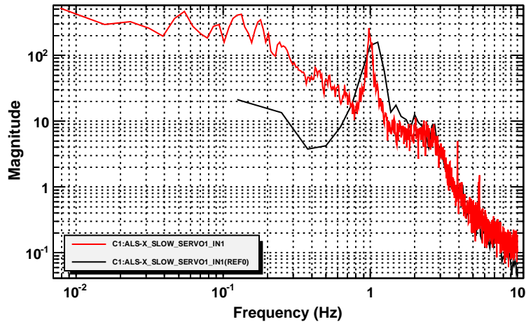
Power spectrum
