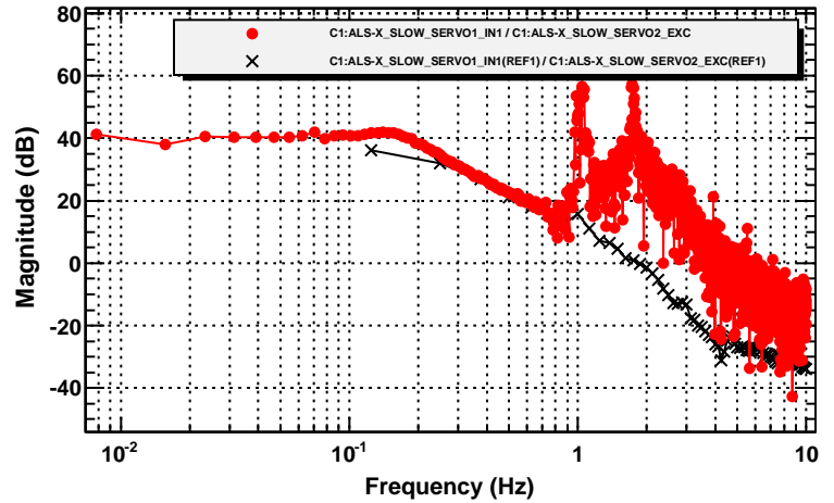
Transfer function
