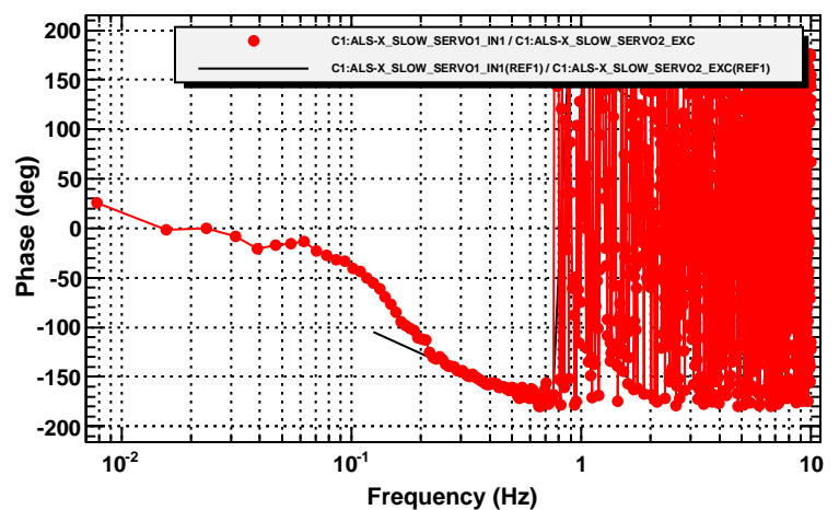
Transfer function
