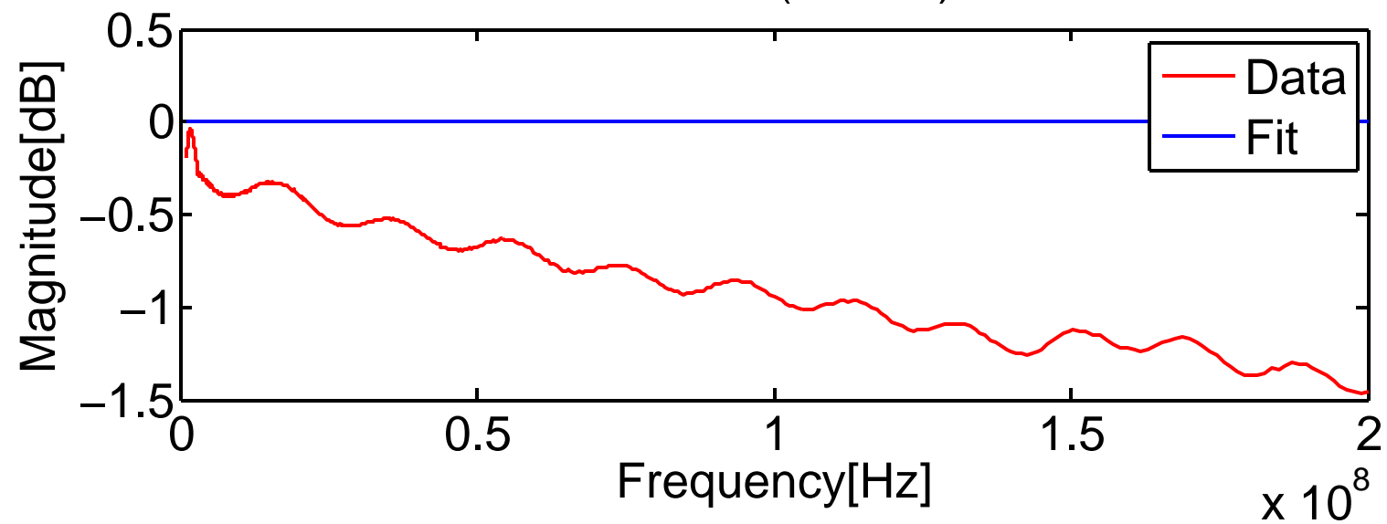
RFcable(550cm)
