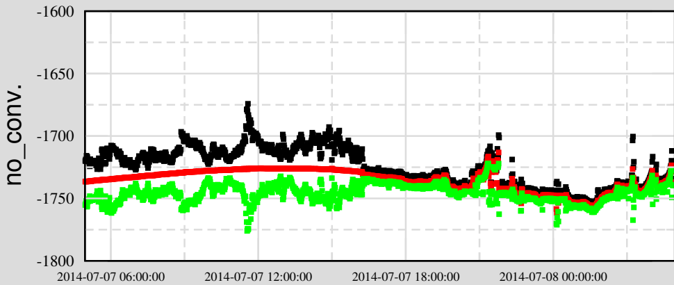
Ch 8: C1:SUS-MC1_SUSPIT_INMON
