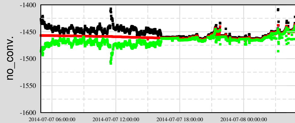
Ch 12: C1:SUS-MC2_SUSYAW_INMON
