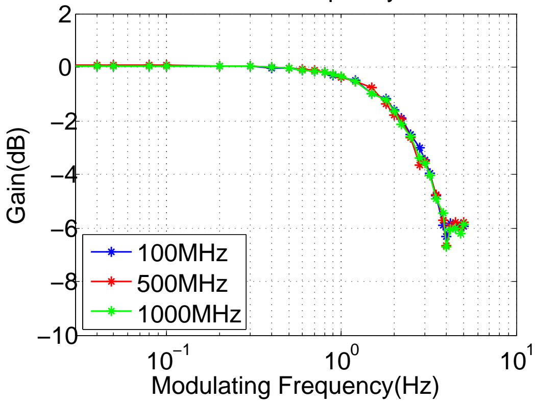
Gain vs Frequency
