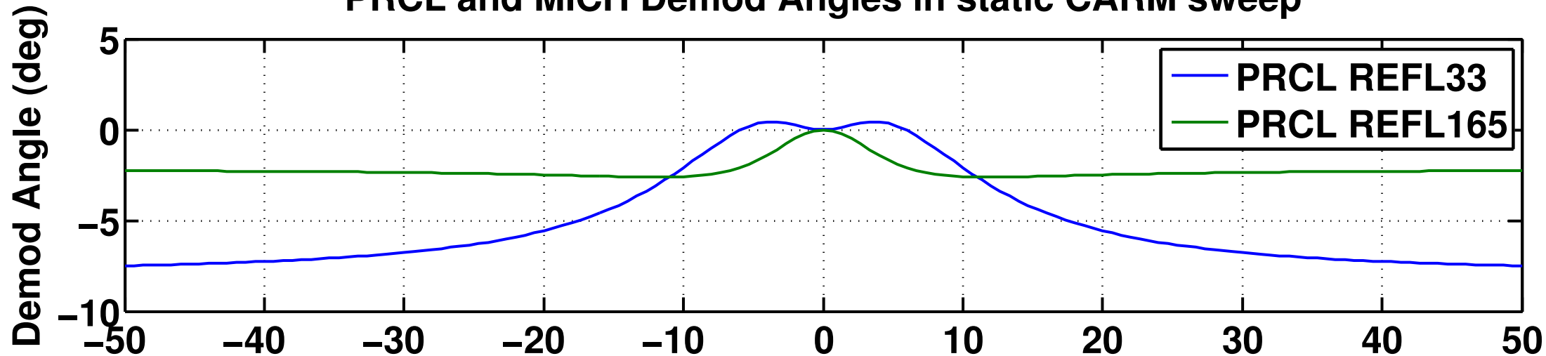
PRCL and MICH Demod Angles in static CARM sweep
