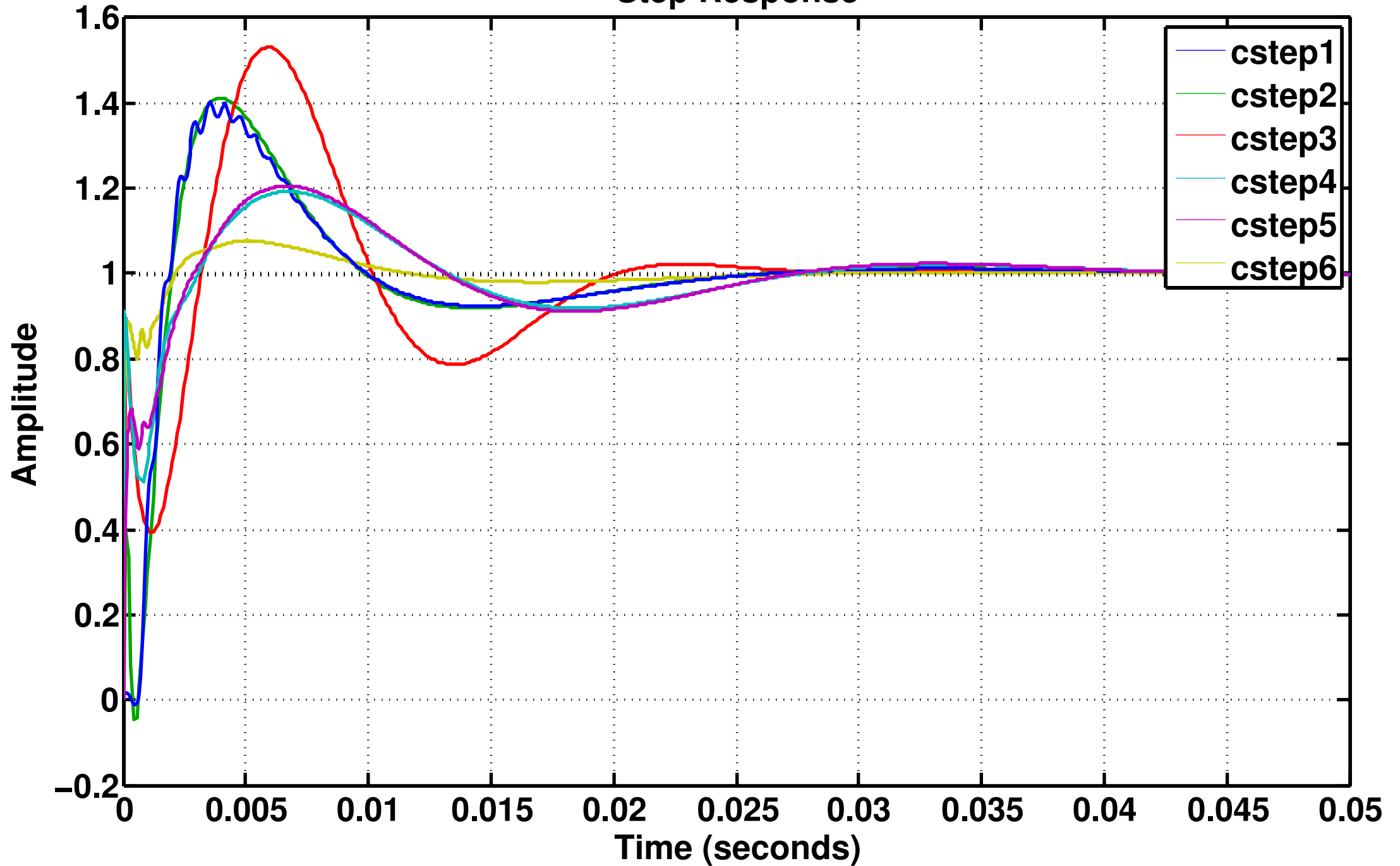
Step Response
