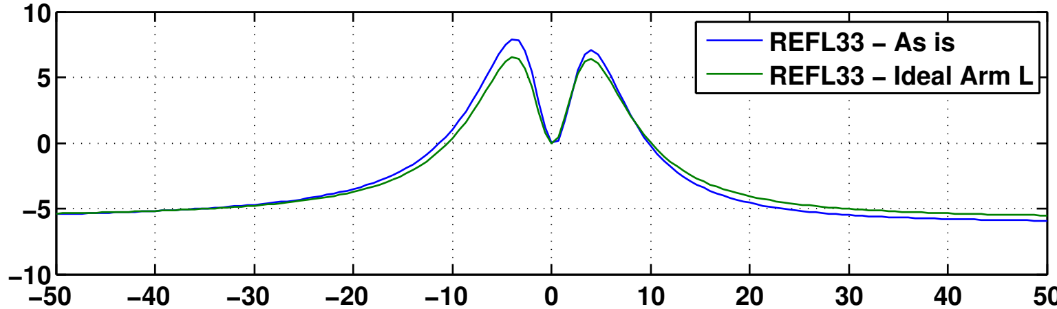
PRCL Demod Angles in static CARM sweep
