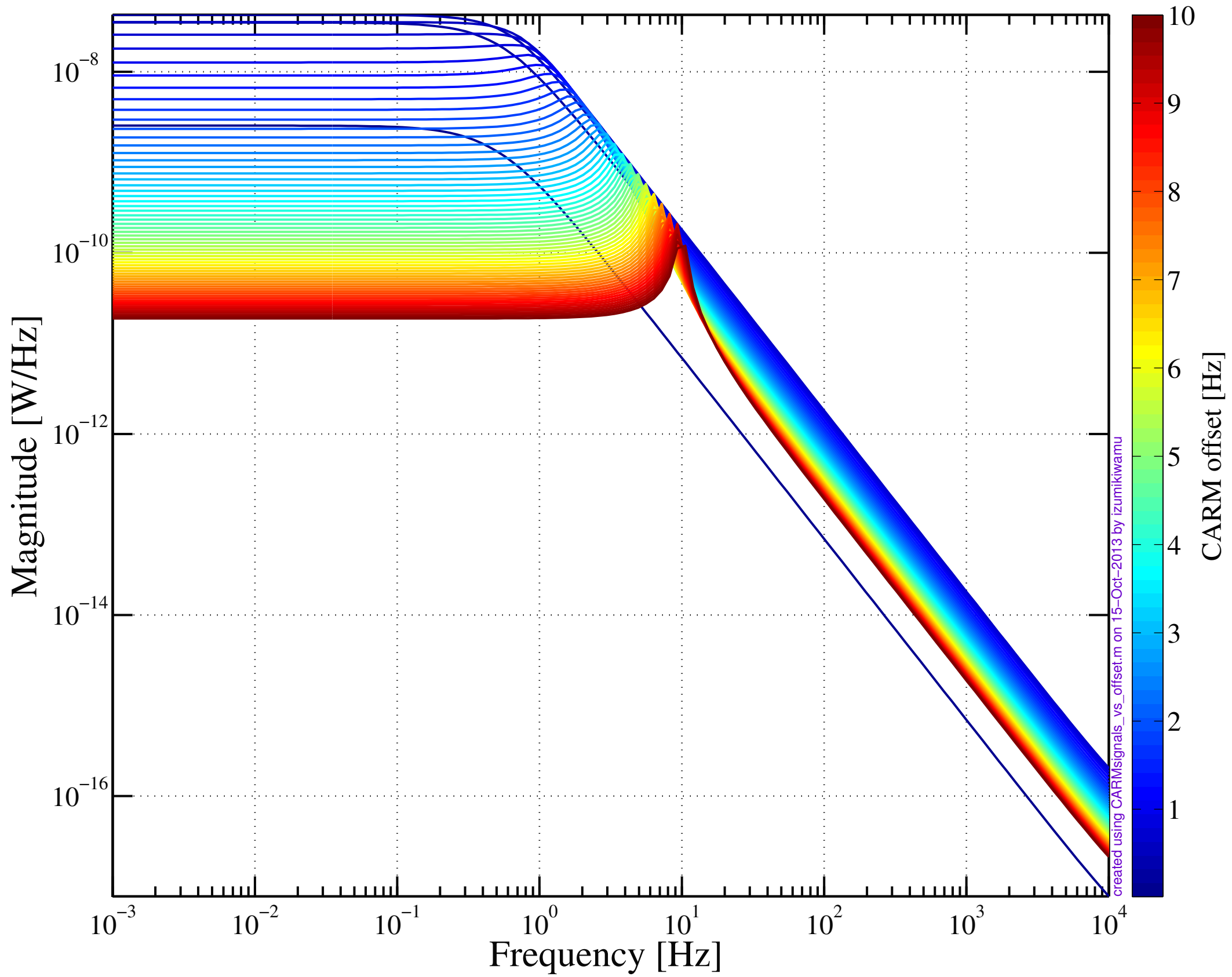
CARM optical gain at TRX DC with various CARM offsets
