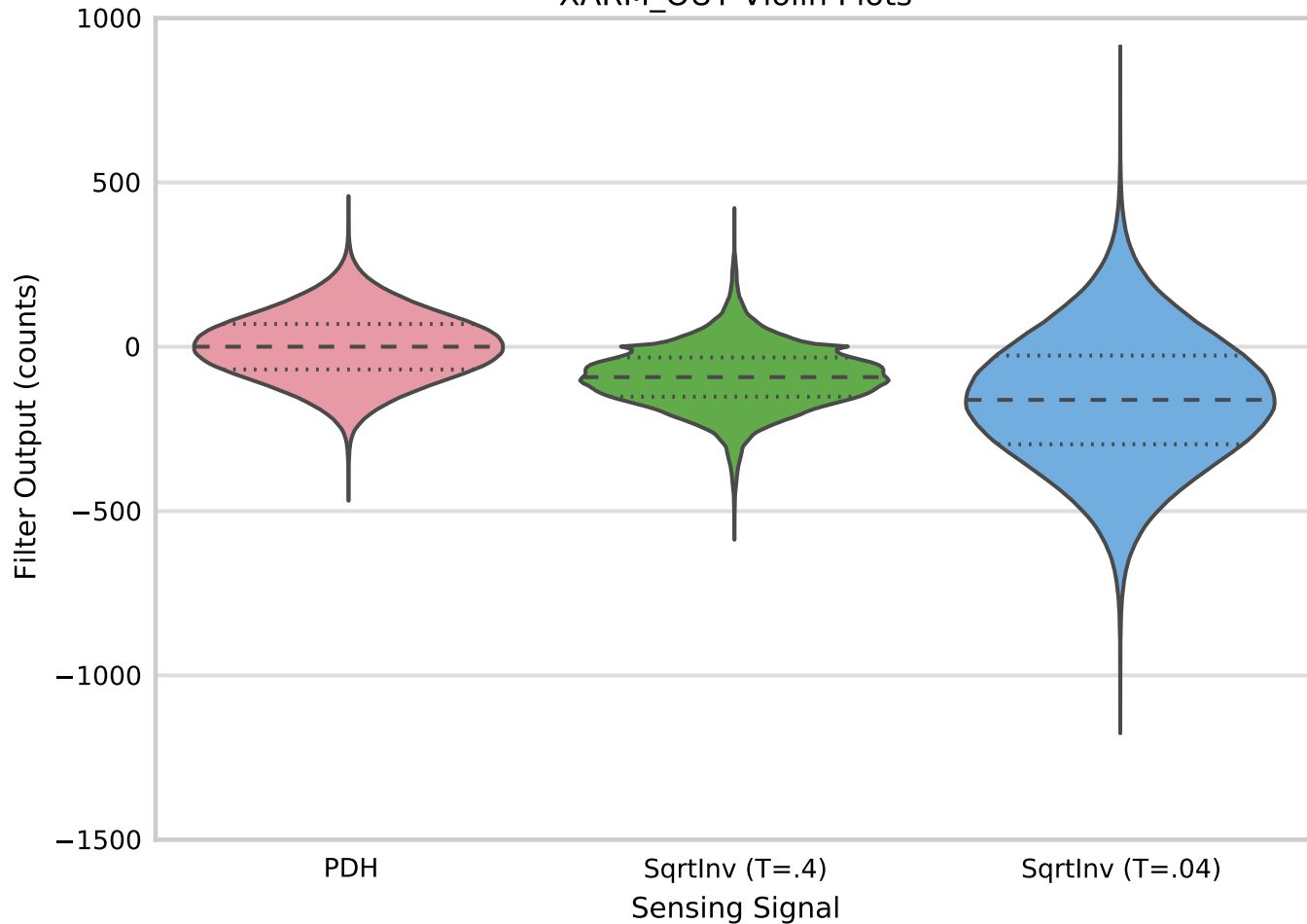
XARM_OUT Violin Plots
