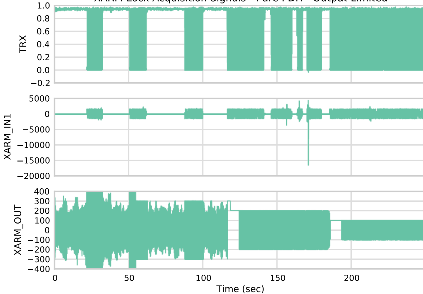
XARM Lock Acquisition Signals - Pure PDH - Output Limited
