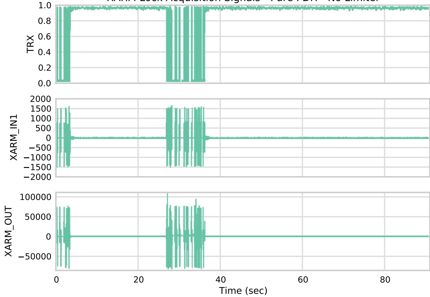
XARM Lock Acquisition Signals - Pure PDH - No Limiter
