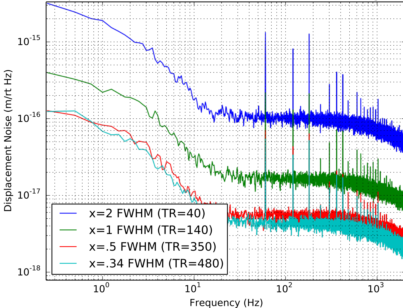
Displacement noise from QPD Dark Noise in SQRTINV signals
