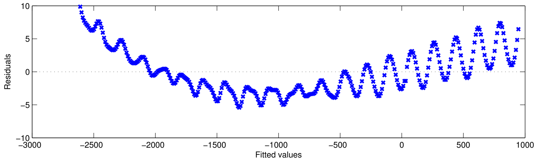
Plot of residuals vs. fitted values
