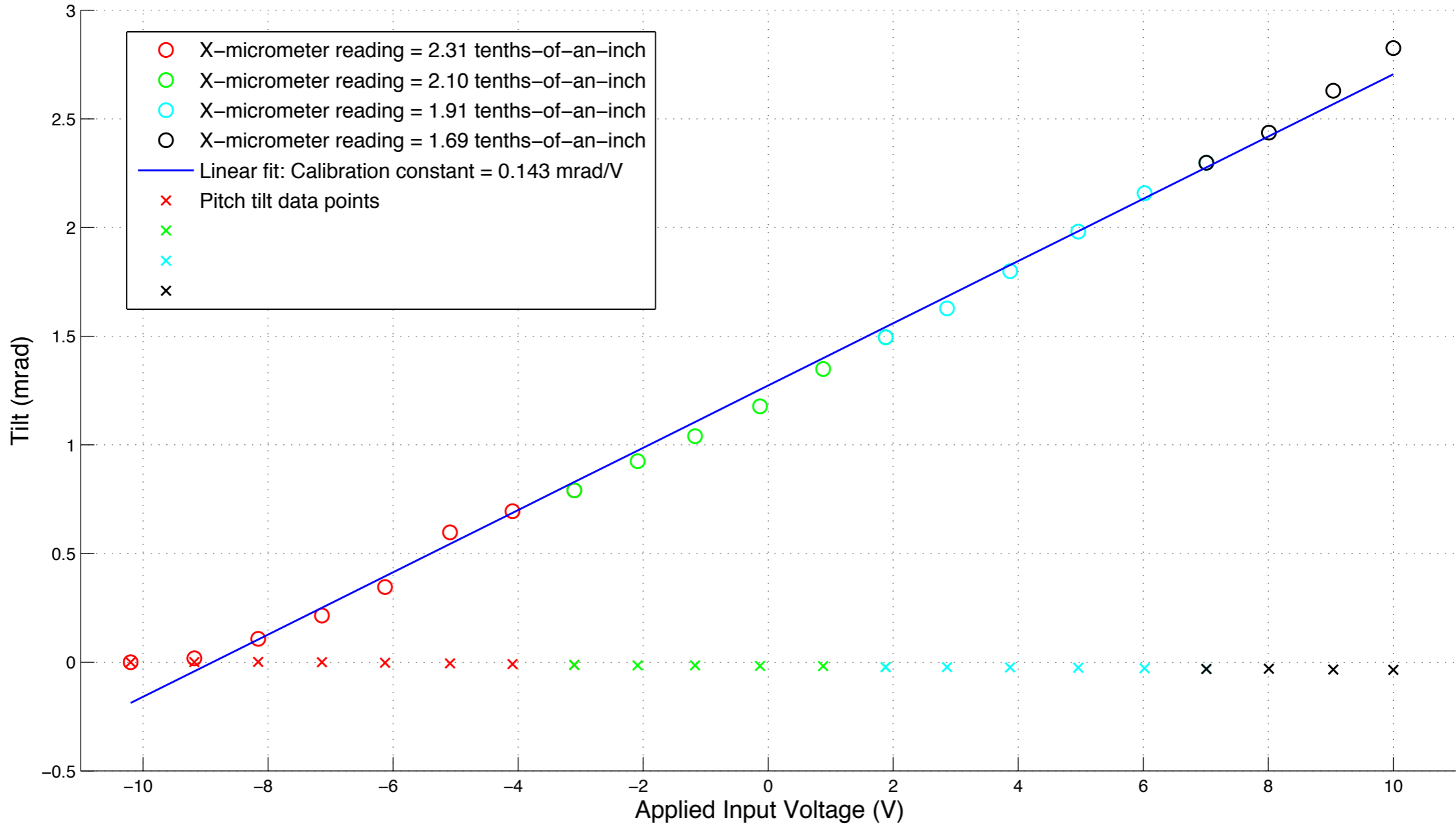
Mirror #1 PZT Calibration – Input to Piezo Yaw (CH1)
