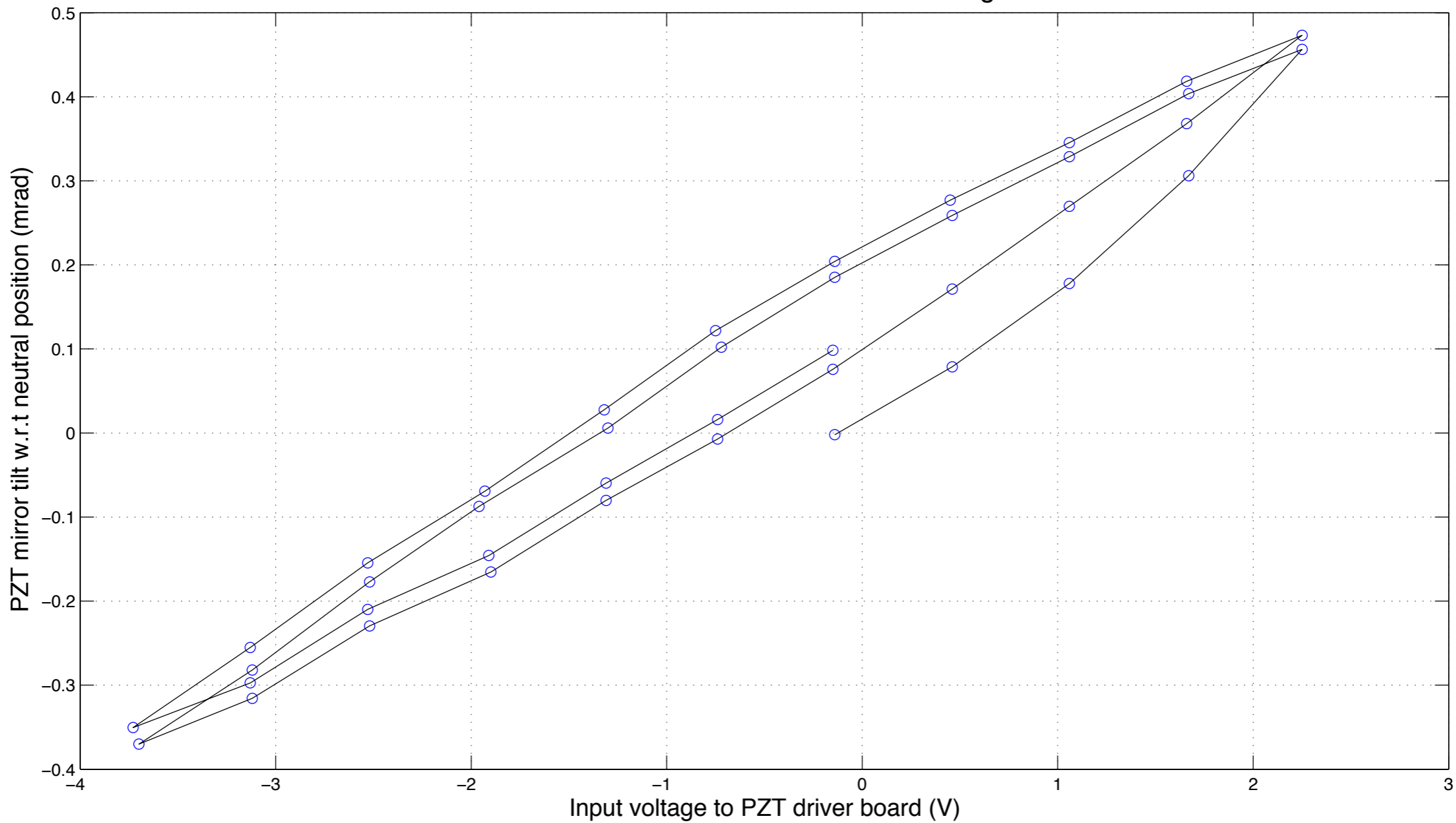
PZT Calibration–In QPD's Linear Range
