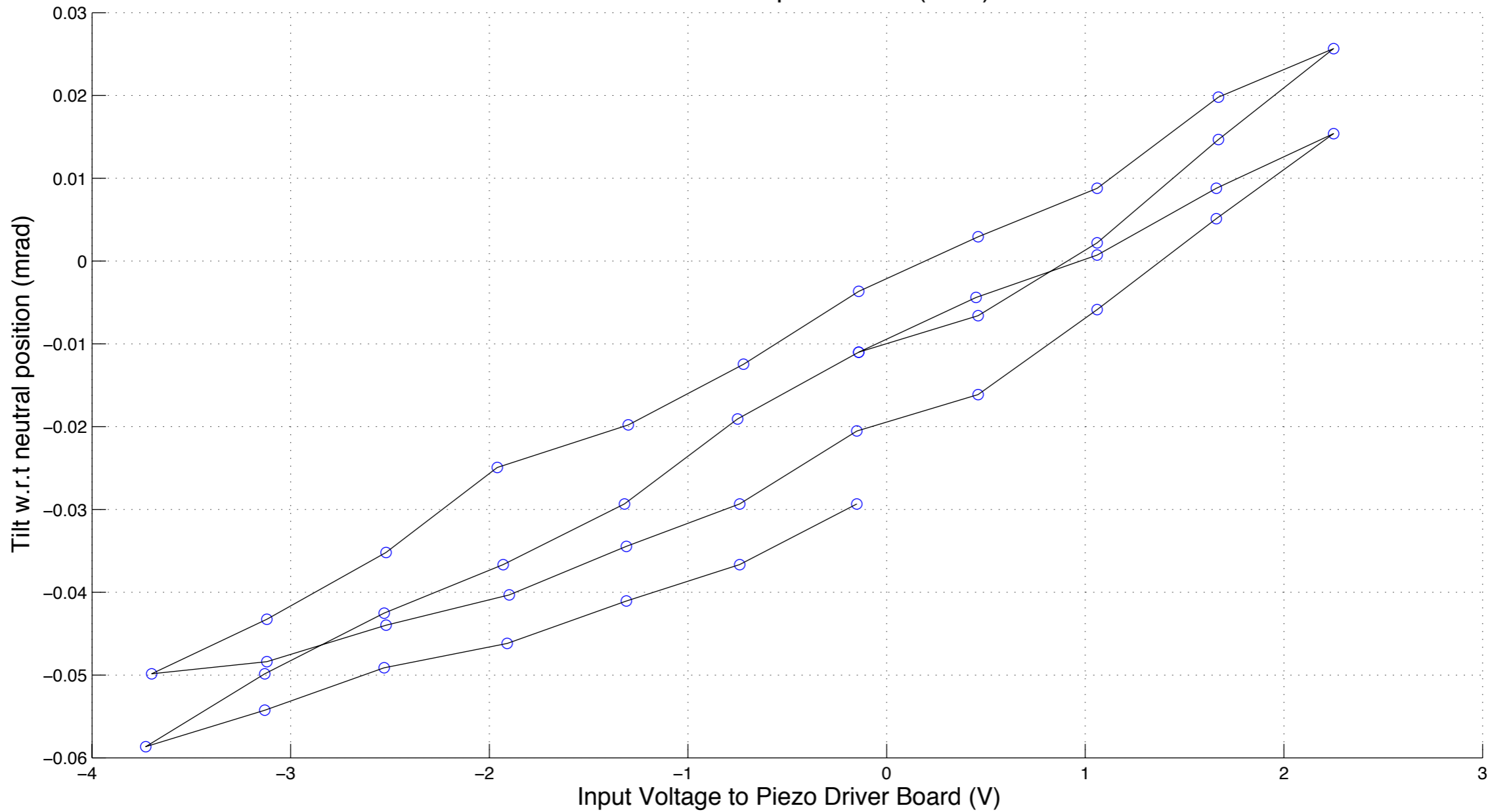
Piezo Calibration with Input to Yaw (CH1)–Pitch tilt
