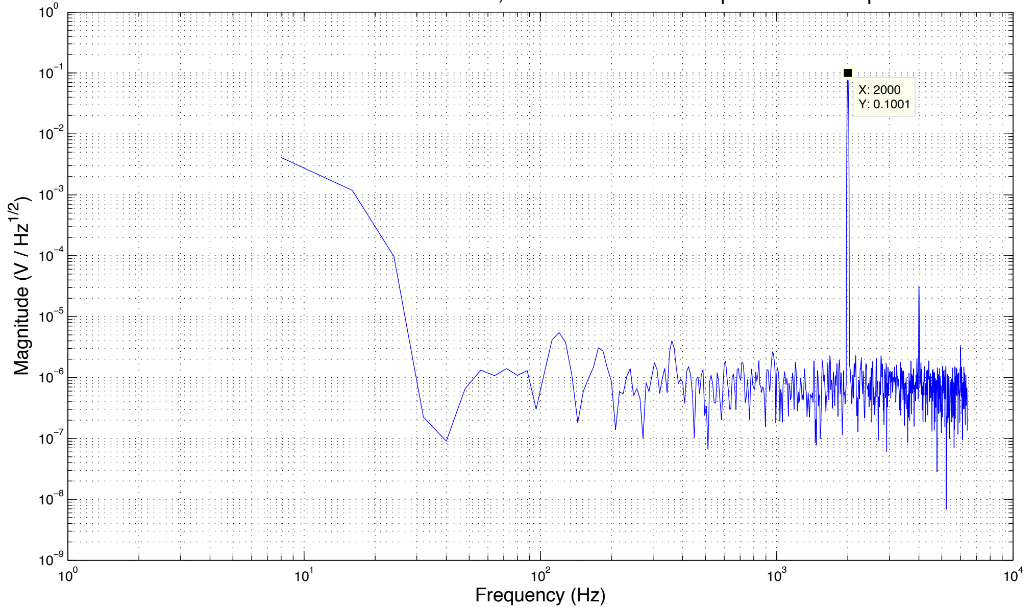
DAC at 1Y4– PSD with 6.4 kHz bandwidth, 2kHz 1000 counts amplitude sine output from Ch9
