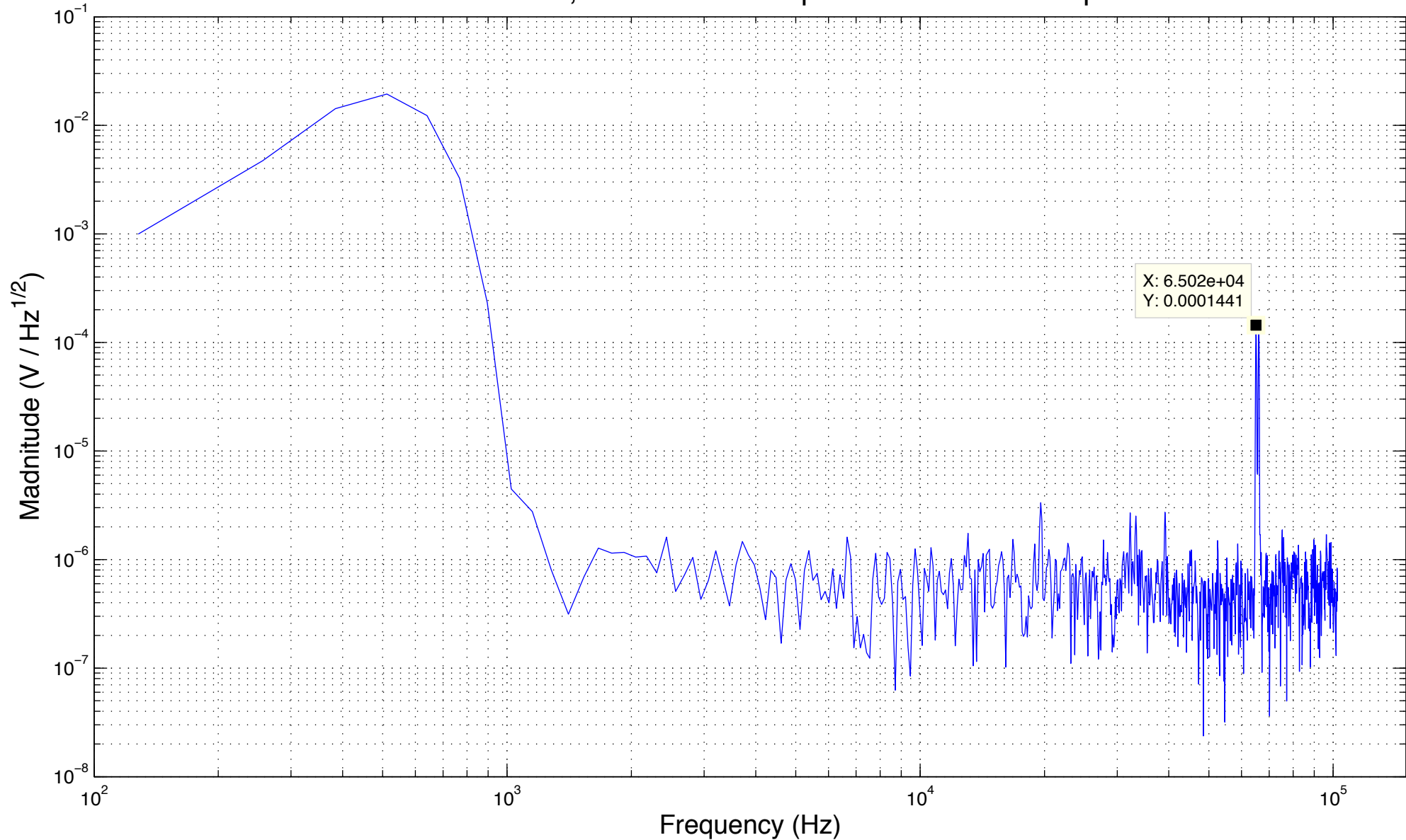
DAC at 1Y4– PSD with 500Hz, 1000 counts amplitude sine wave output from Channel 9
