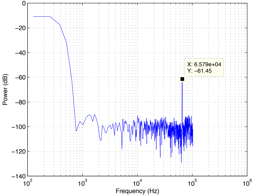
Power Spectrum of DAC at 1Y4 with 200 Hz, 1000 counts amplitude sine wave output
