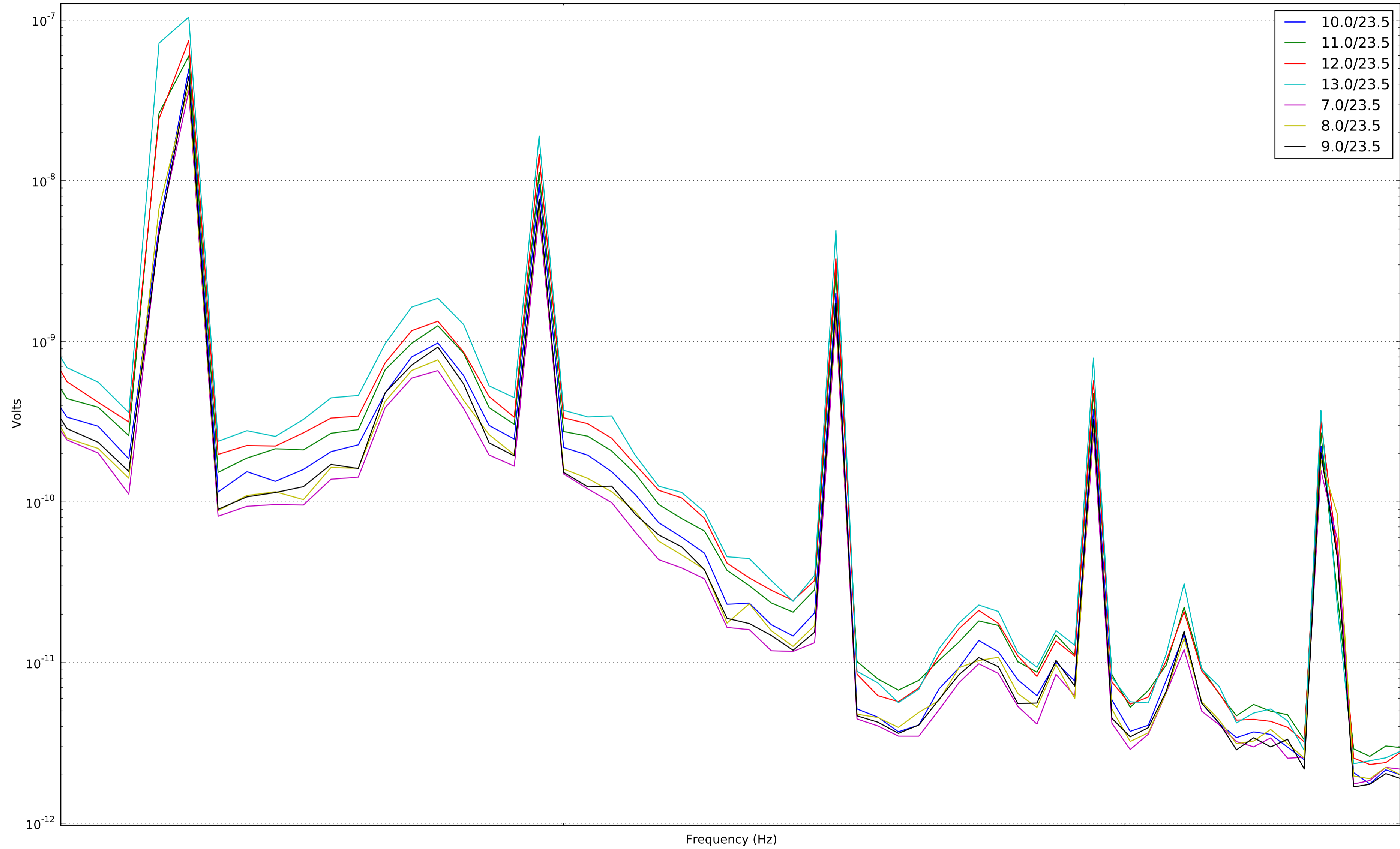
MC error point spectrum
