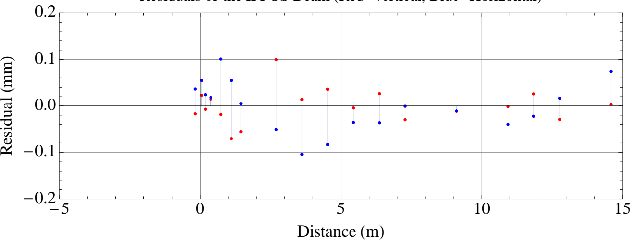
Residuals of the IPPOS Beam (Red=vertical, Blue=Horizontal)
