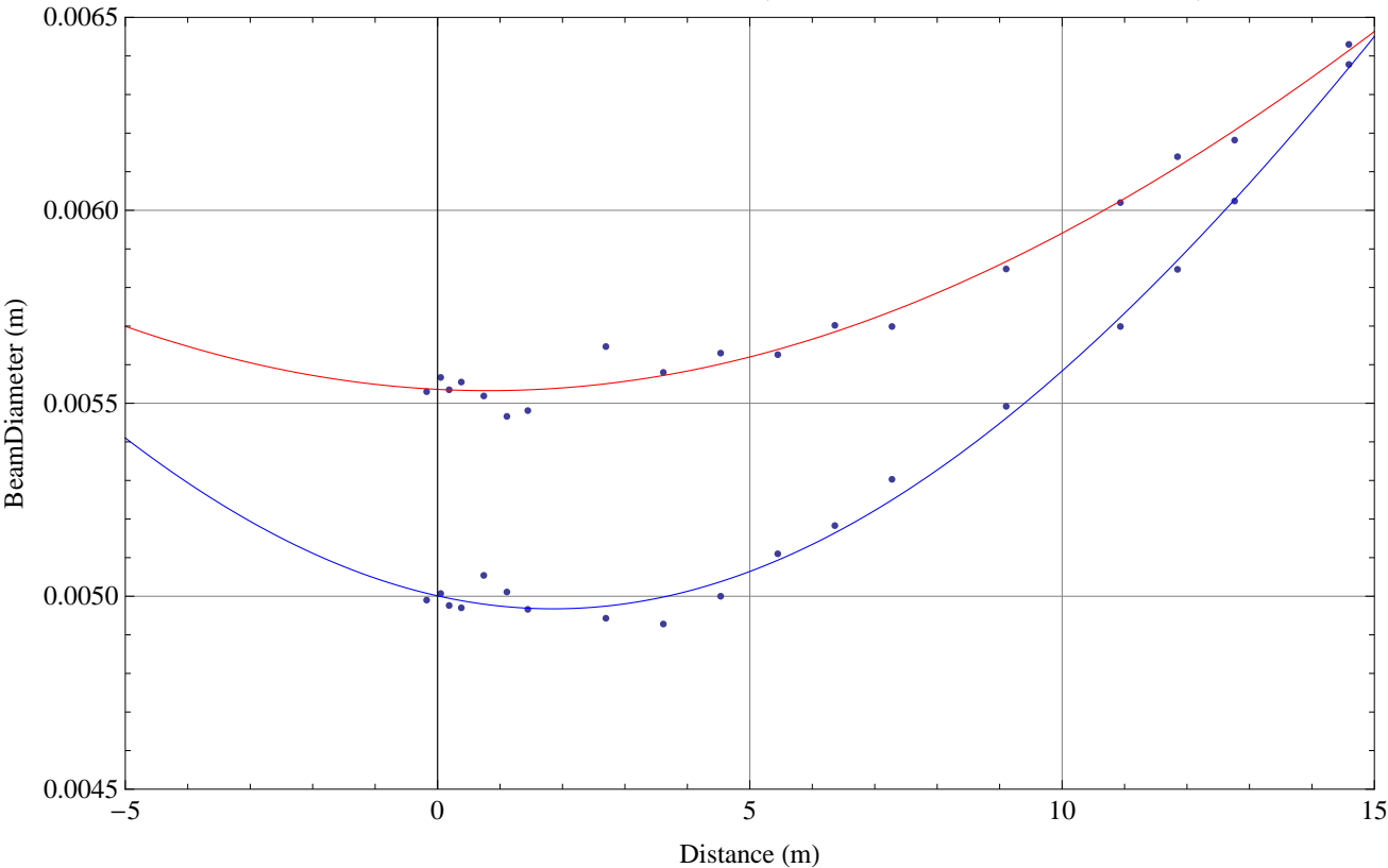
Beam Profile of the IPPOS Beam (Red=vertical, Blue=Horizontal)
