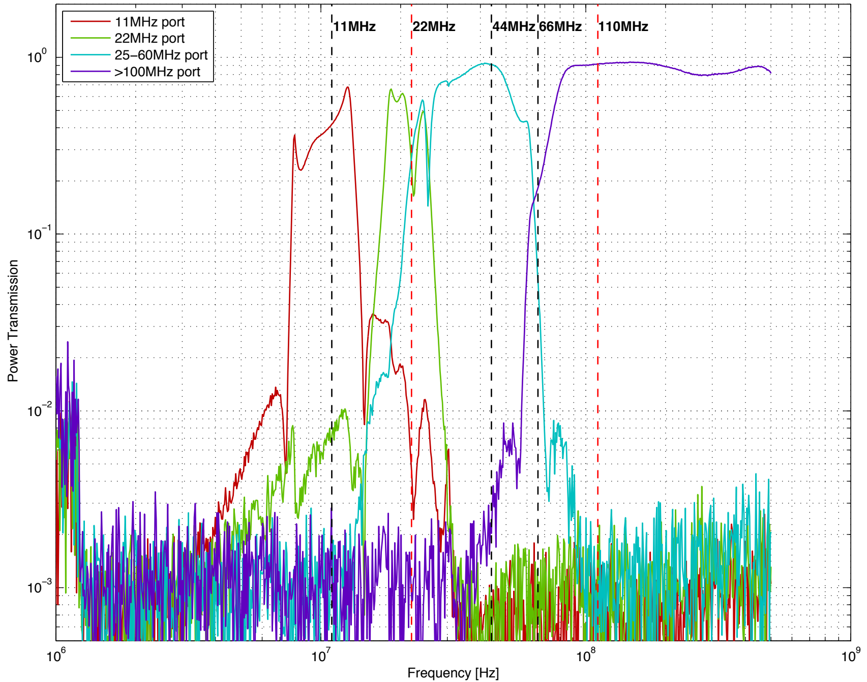
Power Transmission to each output port
