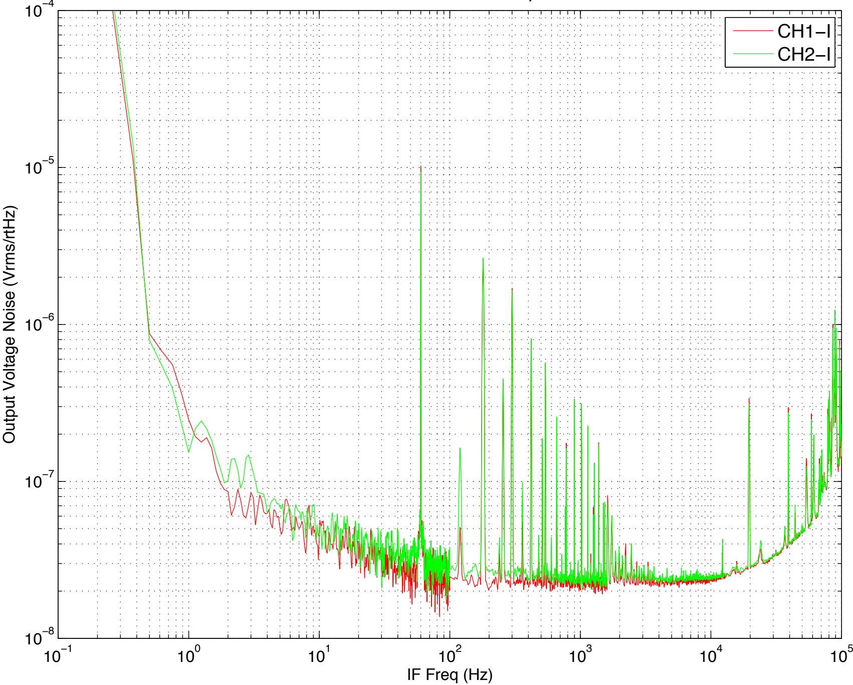
RF Demodulator Test – Output noise
