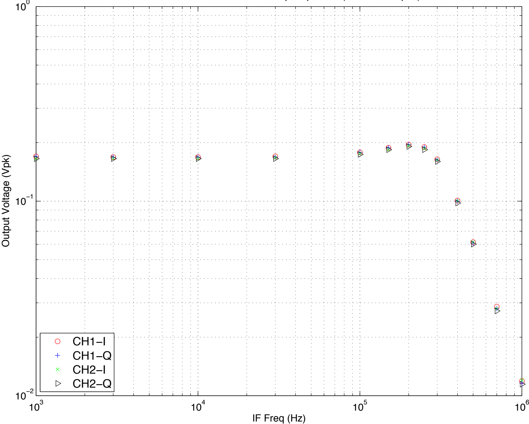
RF Demodulator Test – Freq response (-20dBm input)
