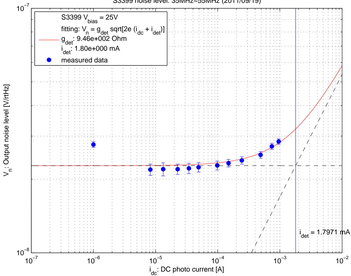
S3399 noise level: 35MHz~55MHz (2011/09/19)
