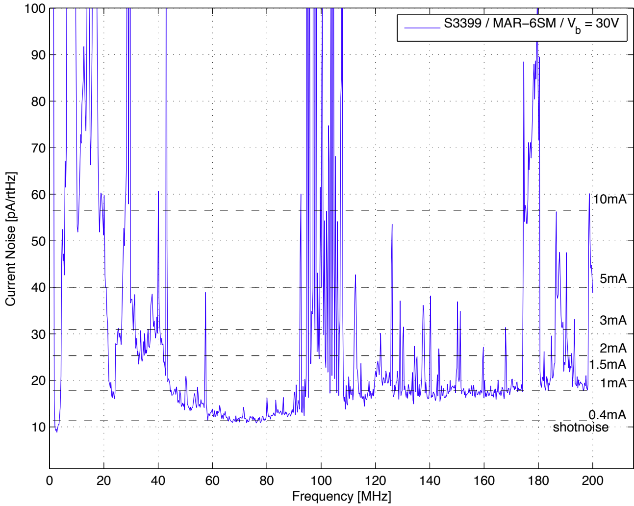
PD current noise level
