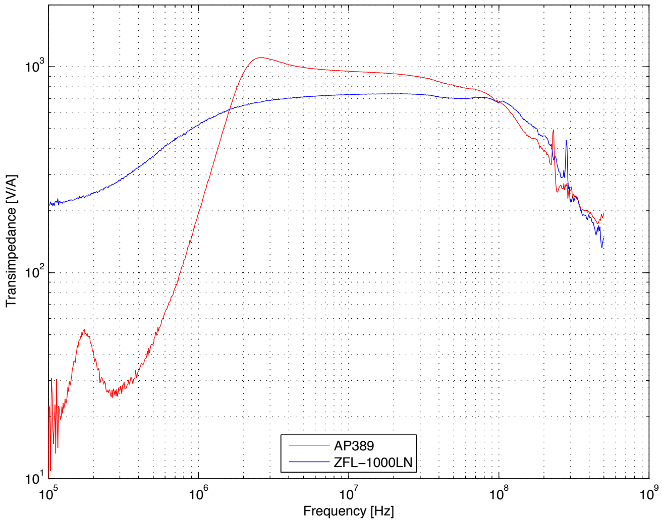
Amplifier comparison
