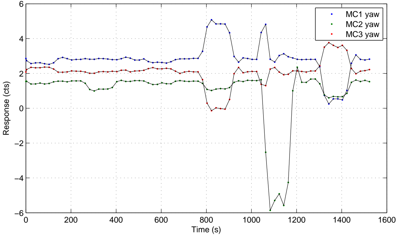
Demodulated MCL response to mirror yaw step
