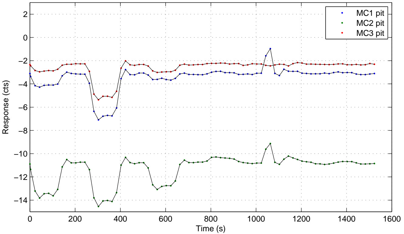
Demodulated MCL response to mirror pitch step
