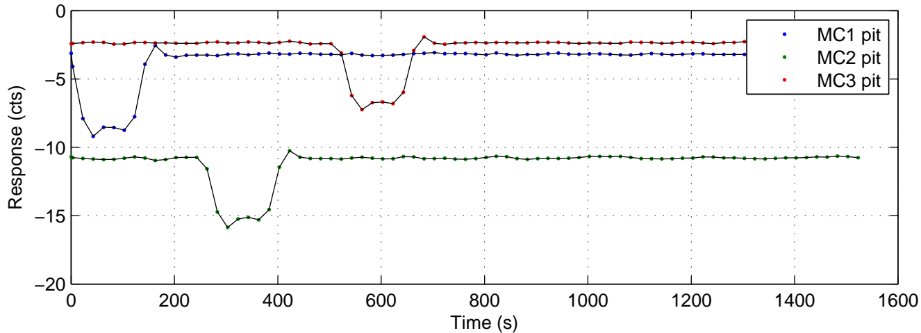
Demodulated MCL response to mirror pitch 10% coil imbalance
