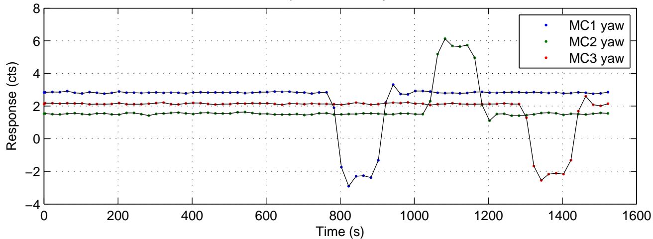
Demodulated MCL response to mirror yaw 10% coil imbalance
