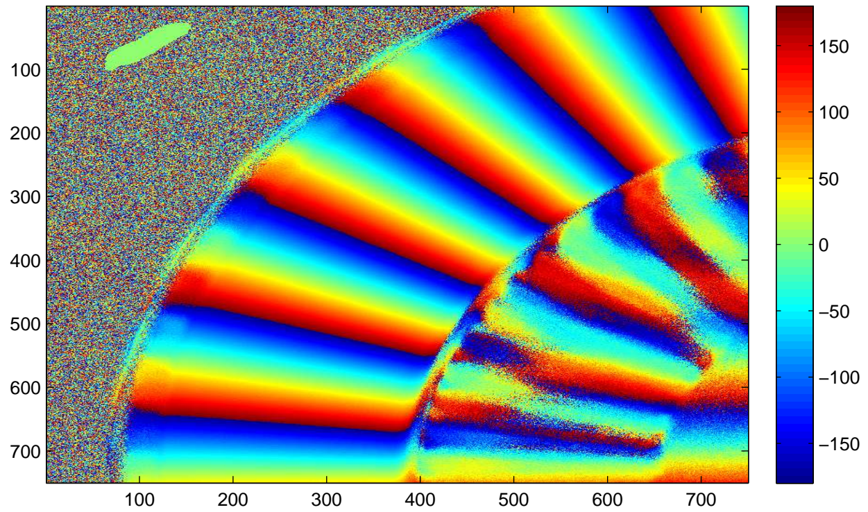
Phase of 25Hz signal (degrees)
