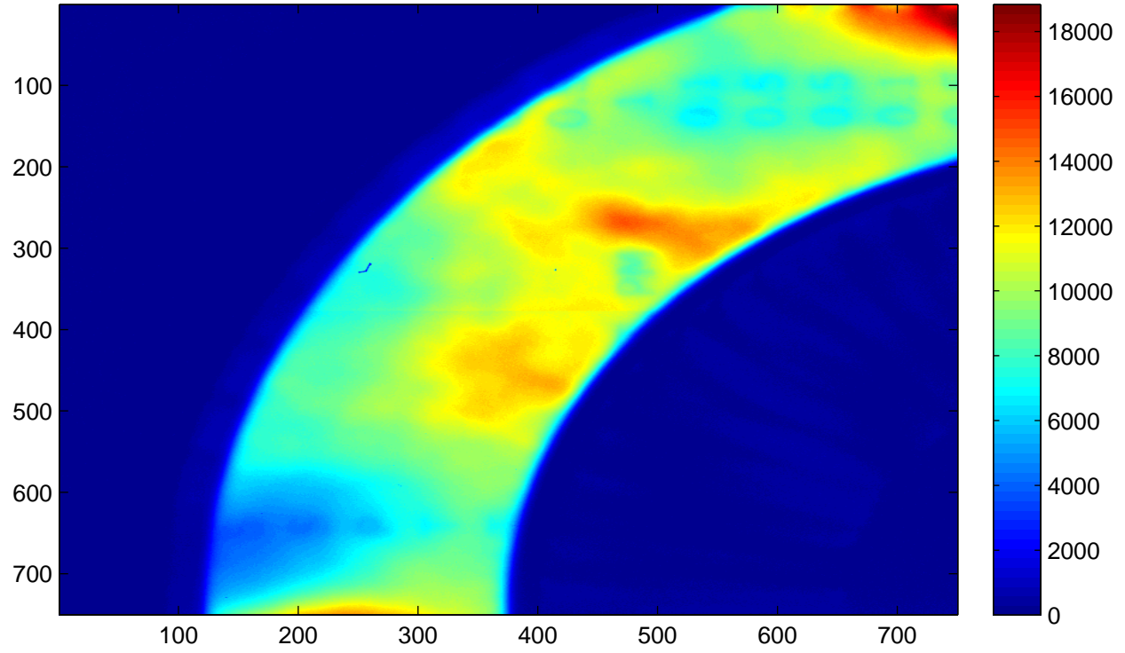
Magnitude of 25Hz signal
