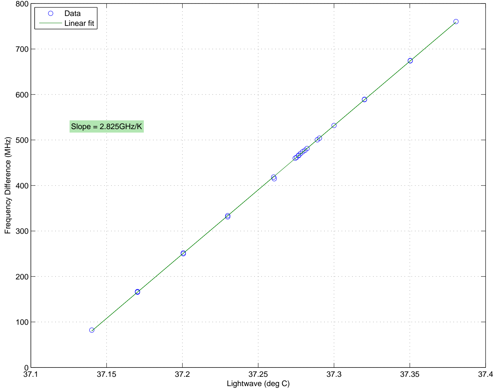
Innolight – Lightwave frequency difference versus LW temperature. Innolight = 39.62 C
