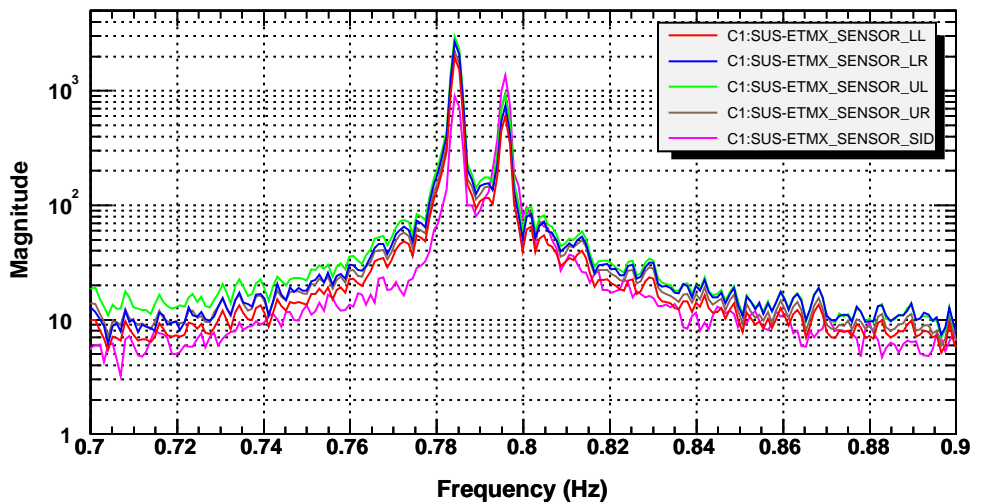
Pendular Modes
