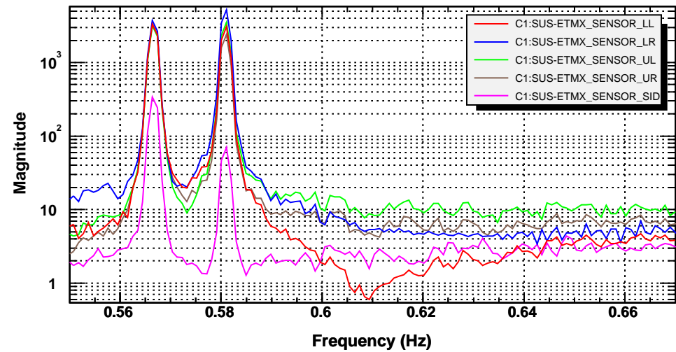
Pitch/Yaw Modes
