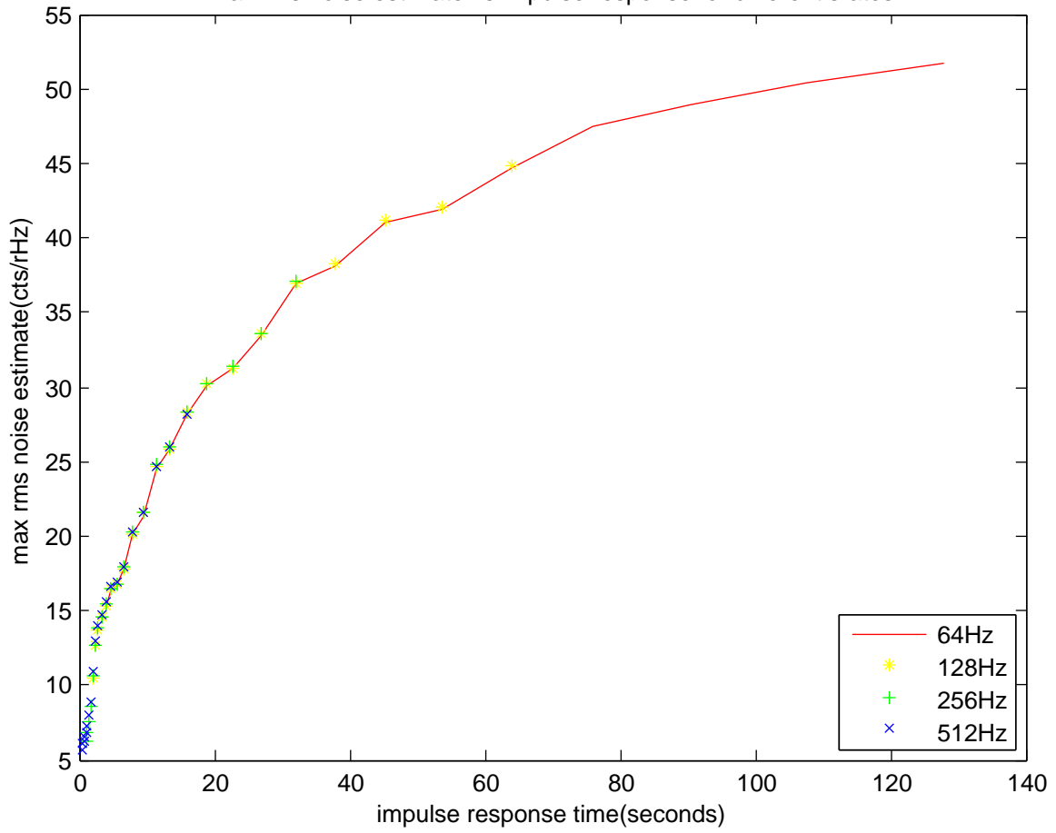
max rms noise estimate vs impulse response for different srates
