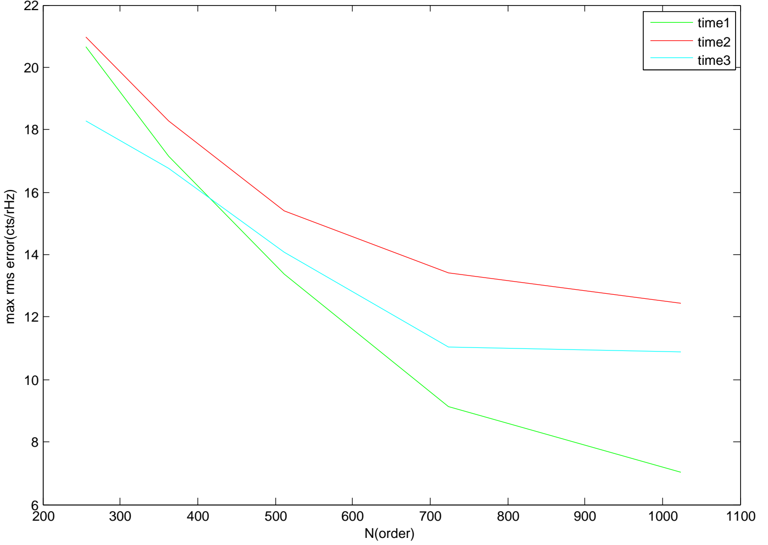
error vs N for different times srates=128
