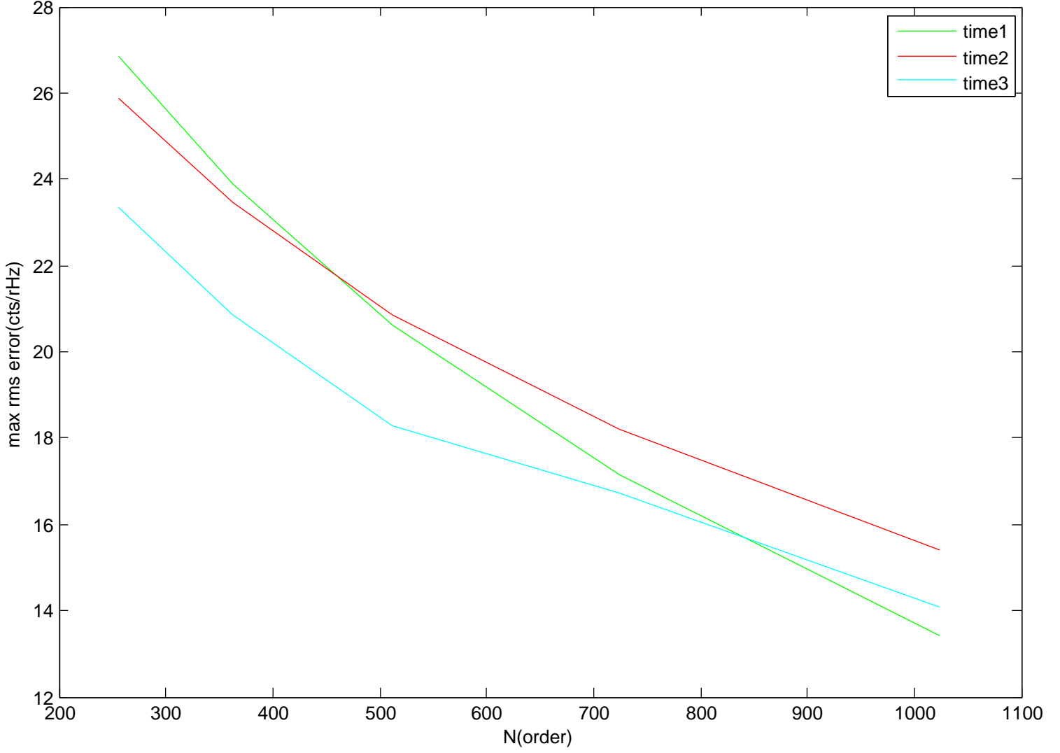
error vs N for different times srate=256
