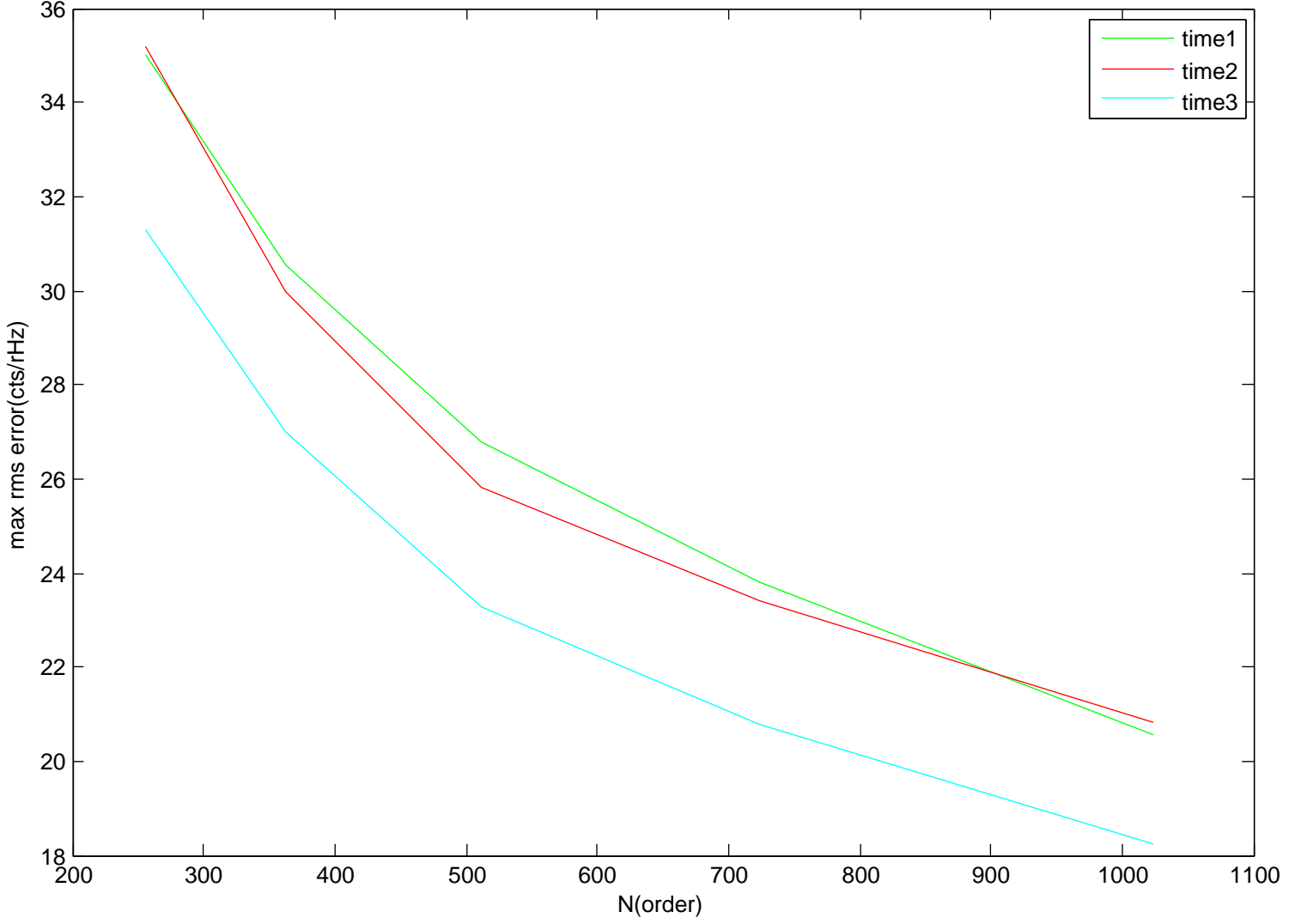
error vs N for different times srate=512
