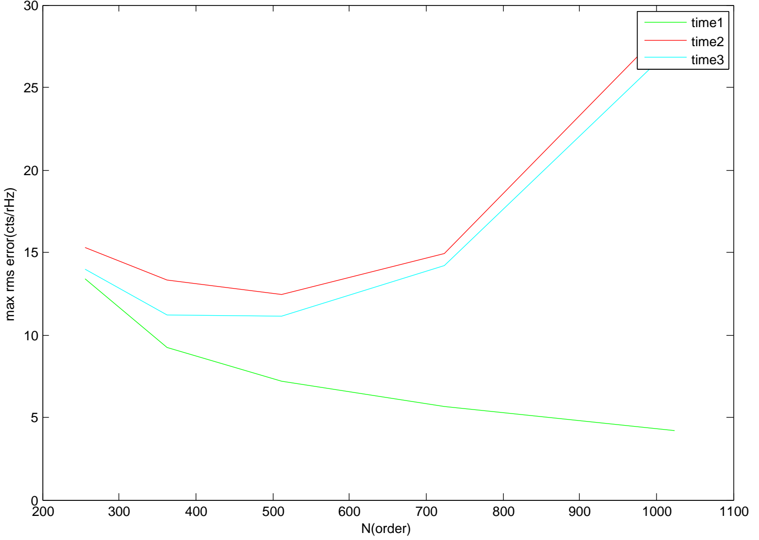
error vs N for different times srate=64
