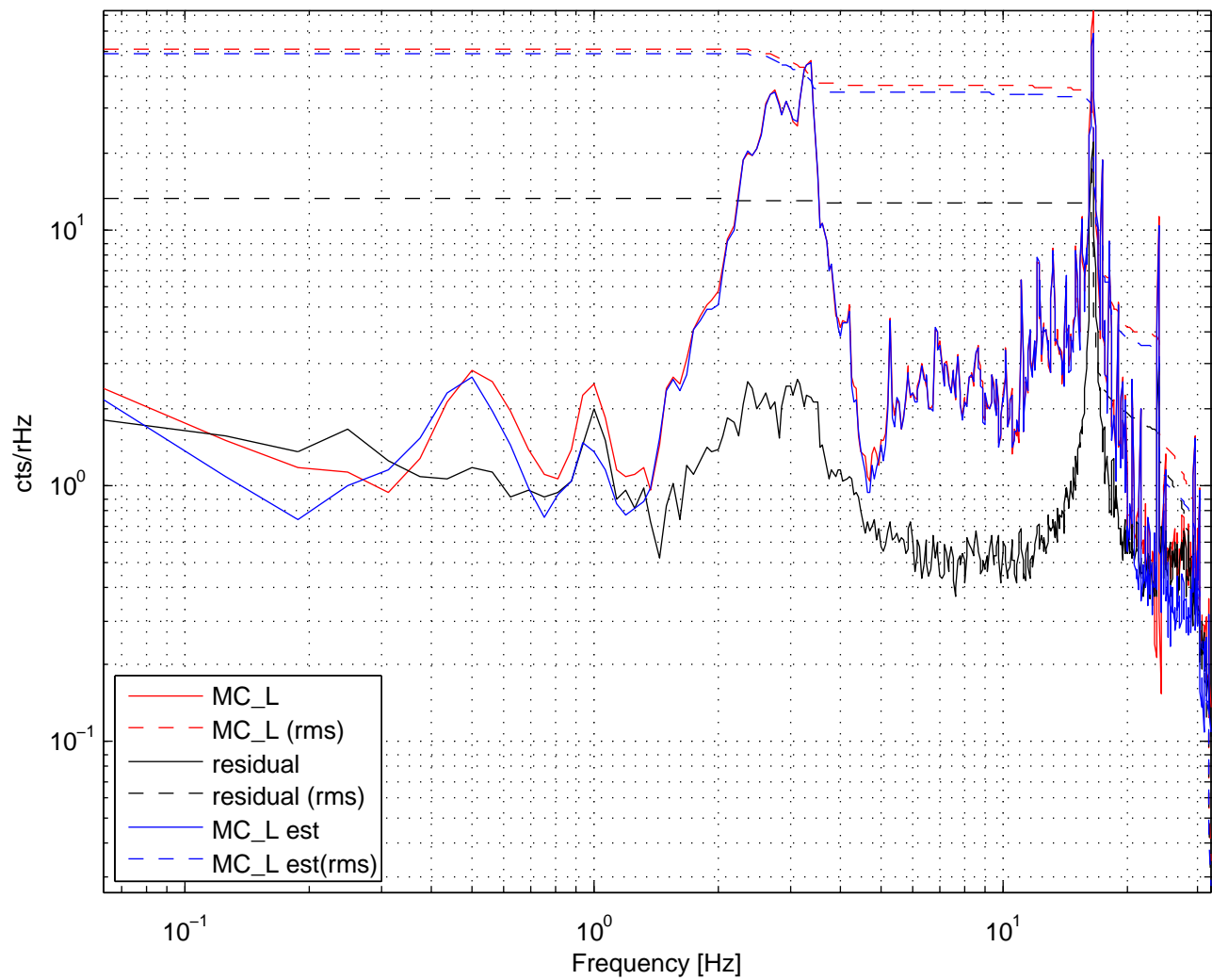
MISO Filter 64Hz N=256
