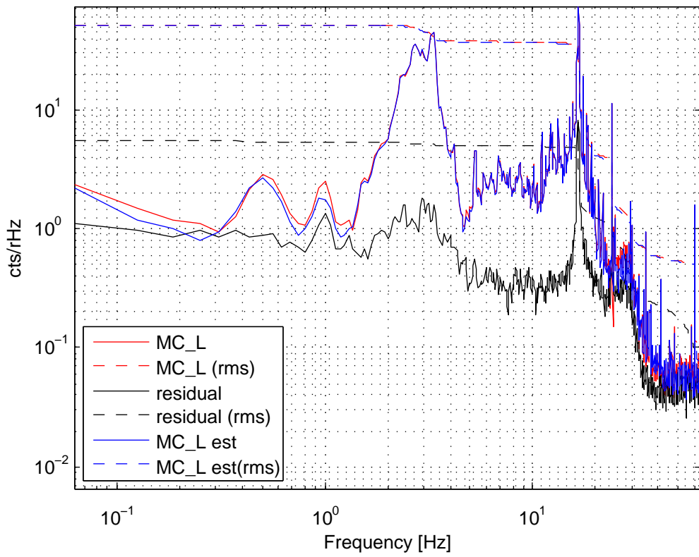
MISO Filter 128Hz N=1448
