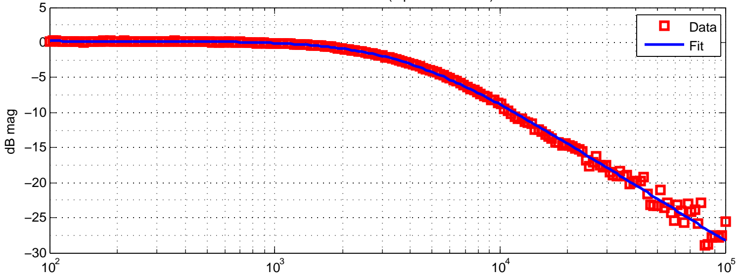
Mode Cleaner TF (1 pole @ 3.8kHz)
