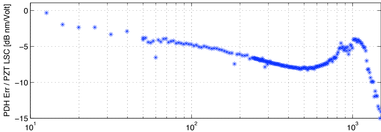
PDH loop response of OMC
