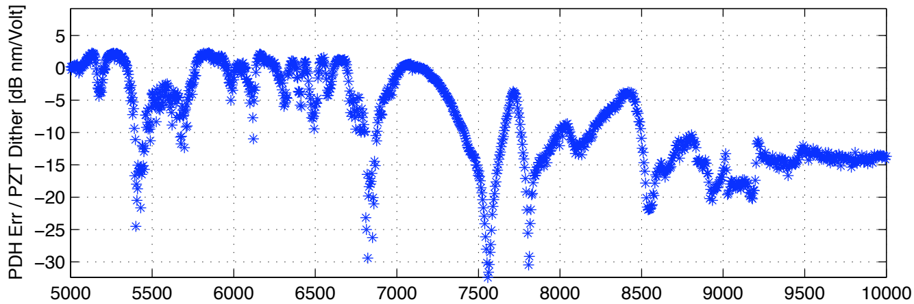
PZT Dither response of OMC
