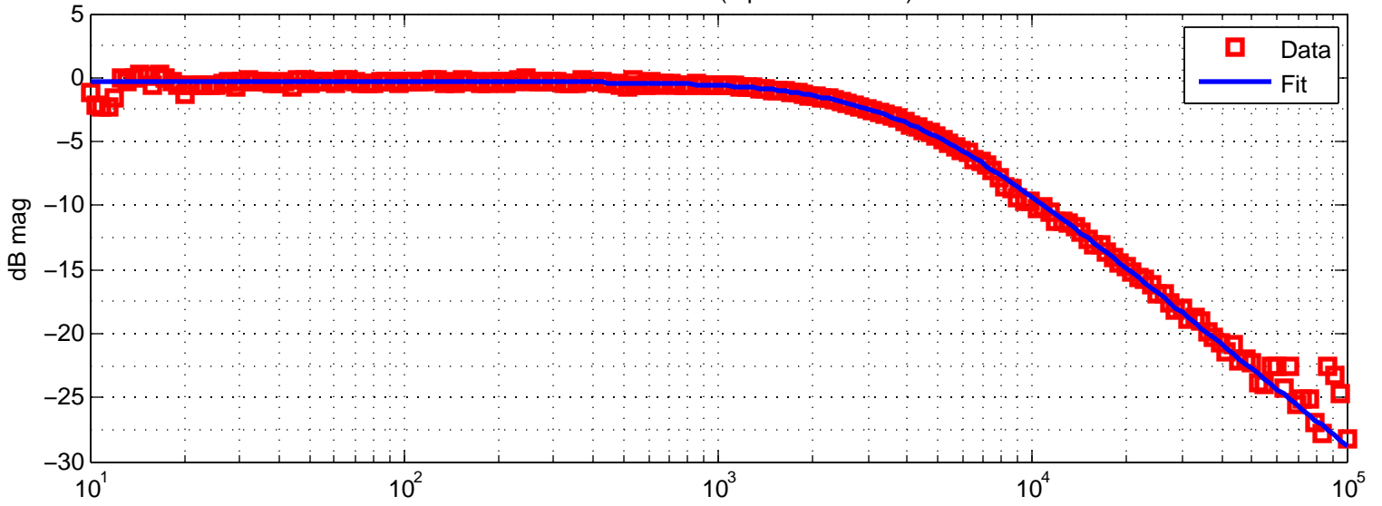
Mode Cleaner TF (1 pole @ 3.8kHz)
