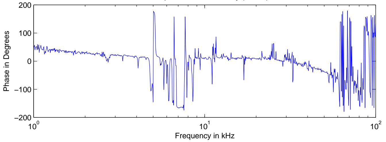
PZT reponse of locked cavity (Phase)
