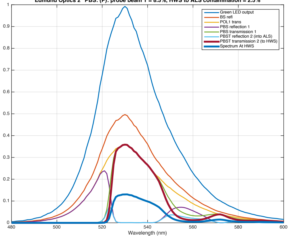
Edmund Optics 2" PBS: (P): probe beam T = 8.3%, HWS to ALS contamination = 2.5%
