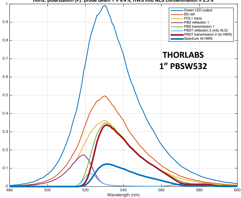
Horiz. polarization (P): probe beam T = 9.4%, HWS into ALS contamination = 2.5%
