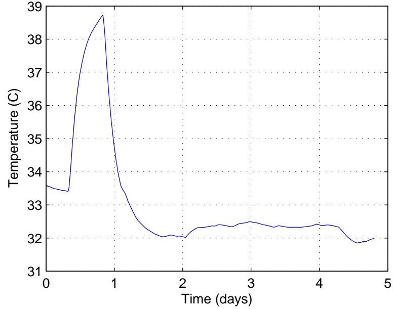
Hartmann plate temperature vs time. End = 30-May-2011 10:28:44
