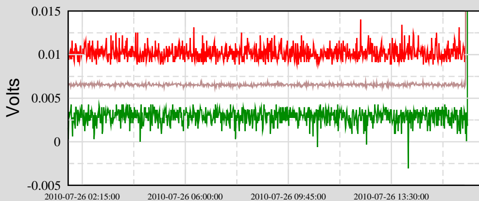
Ch 1: C4:TCS-ATHENA_I_ACTUAL_VOLTS (Actual Current to PD)
