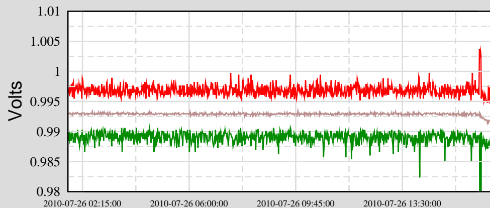
Ch 4: C4:TCS-ATHENA_PD_VOLTAGE (On-board PD output)
