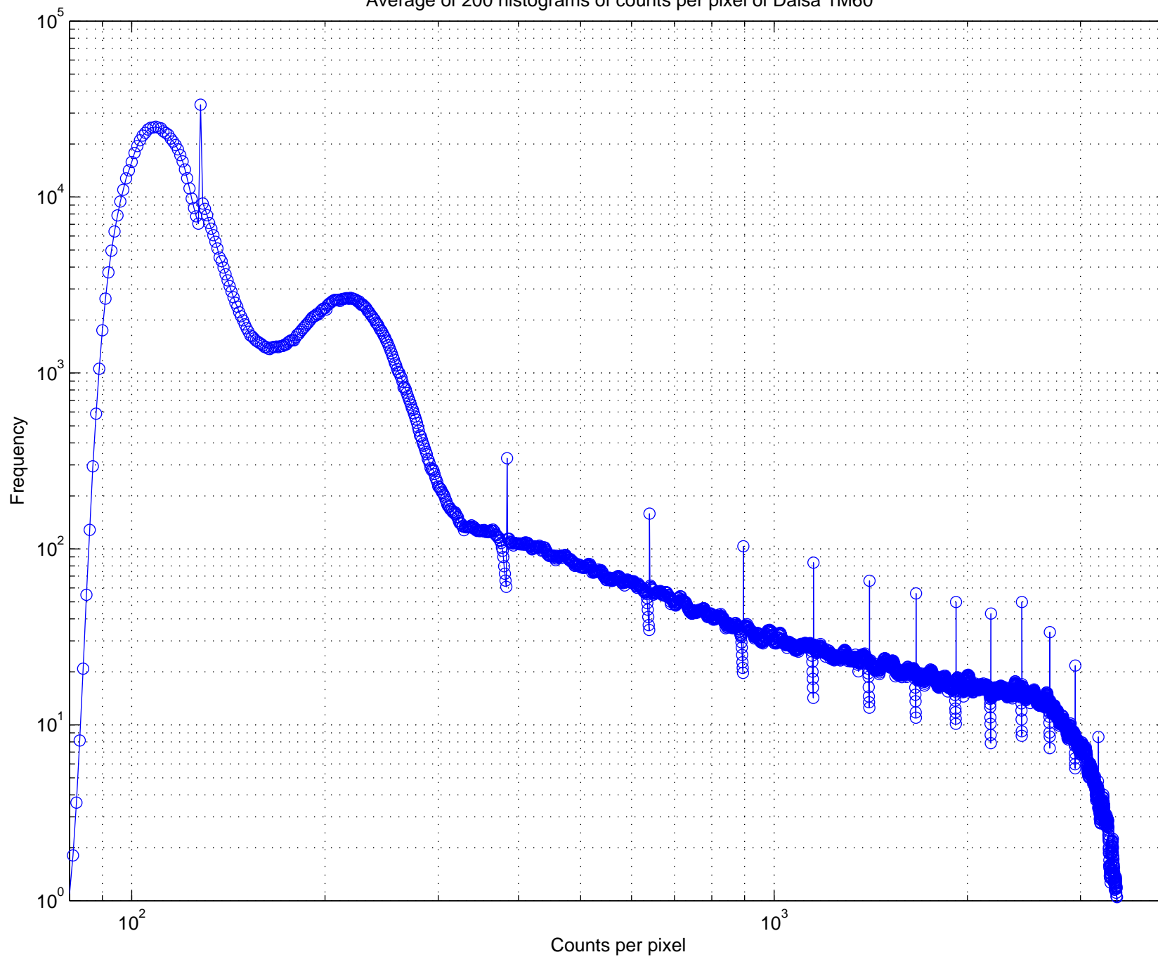
Average of 200 histograms of counts per pixel of Dalsa 1M60
