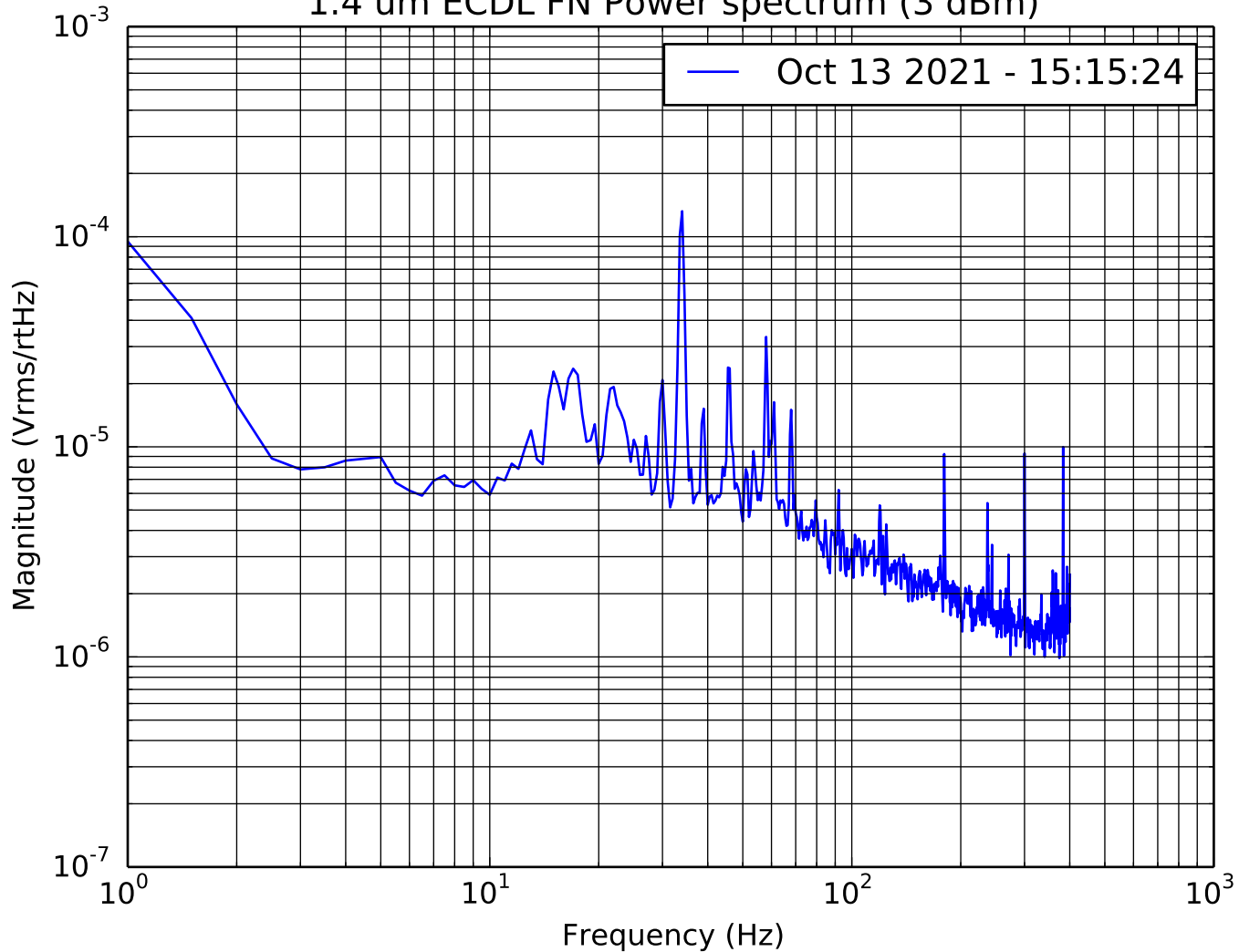
1.4 um ECDL FN Power spectrum (3 dBm)
