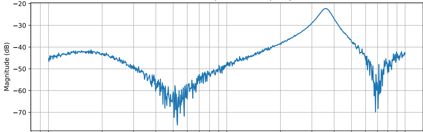
RFPD Transfer Function from test input to test output - Jan 15 2021 - 17:22:12
