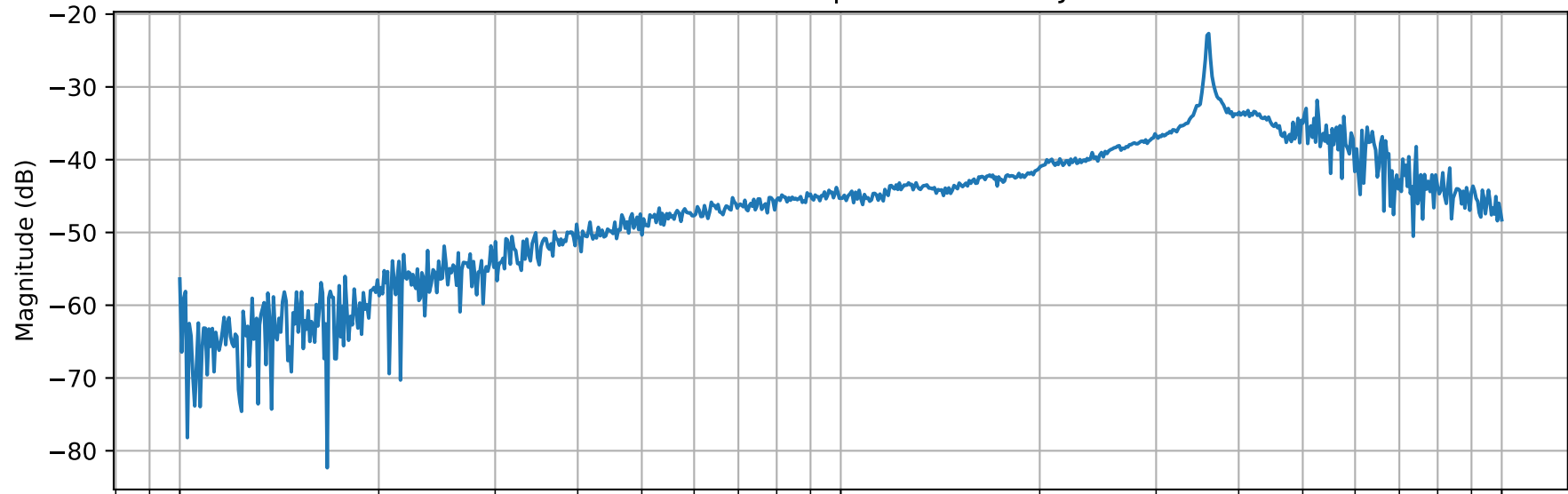
EOM Driver Transfer Function from input to RF Mon - Jan 15 2021 - 15:12:44
